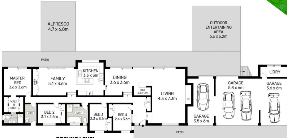
GROUND LEVEL
